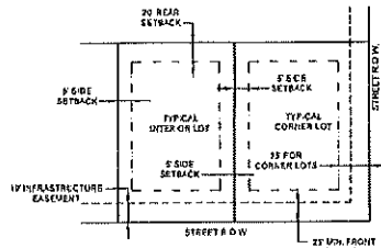
TYPICAL LOT DETAIL FOR LOTS 17-49 N.T.S.
